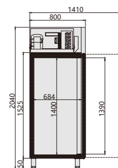
侧视图 Side View
